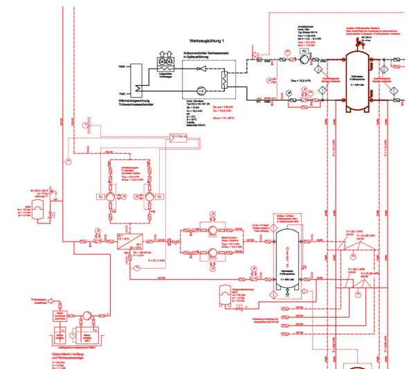
Excerpt: R+I diagram of the refrigeration supply for tool cooling
